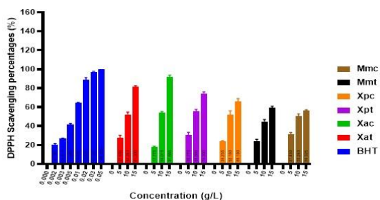
Figure 3: DPPH scavenging properties of essential oils. BHT: Butyl Hydroxy Toluene; MMT= Monodora myristica of Chad; Mmc= Monodora myristica of Cameroon; Xpt= Xylopiya parviflora of Chad; Xpc= Xylopiya parviflora of Cameroon; Xat= Xylopiya aethiopicia of Chad; Xac= Xylopiya aethiopicia of Cameroon
