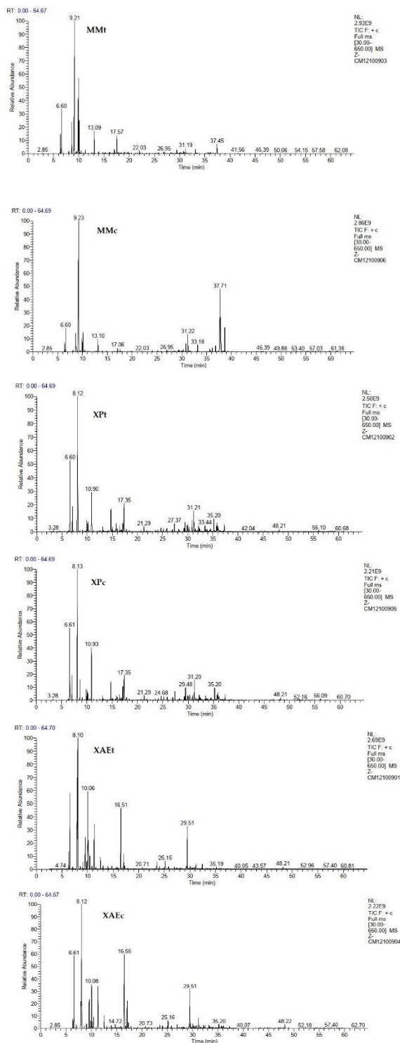
Figure 1. Total ion chromatogram of essential oils using GC-MS. The GC/MS system used is the HEWLETT-PACKARD 589 0 series II, equipped with a capillary column of fused silica 30 m x 0.25 mm and a grafted stationary phase of type HP5 (5%-phenylmethylpolysiloxane). The mass detector is a quadrupole type (Model 5972) and the ionization energy used is 70 eV. MMt= Monodora myristica from Chad; MMc= Monodora myristica from Cameroon; XPt= Xylopia parviflora of Chad; XPc= Xylopia parviflora of Cameroon; XAEt= Xylopia aethiopica from Chad; XAEc= Xylopia aethiopica from Cameroon.
